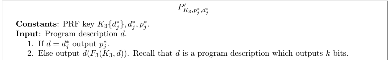
Figure 12: Program P'_{K_3, p_j^*, d_j^*}
