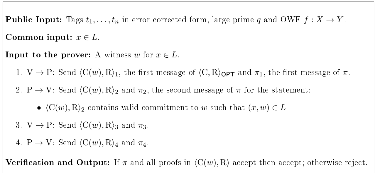
Figure 5: The 4-round non malleable zero-knowledge argument of knowledge protocol \langle \text{P}, \text{V} \rangle .
