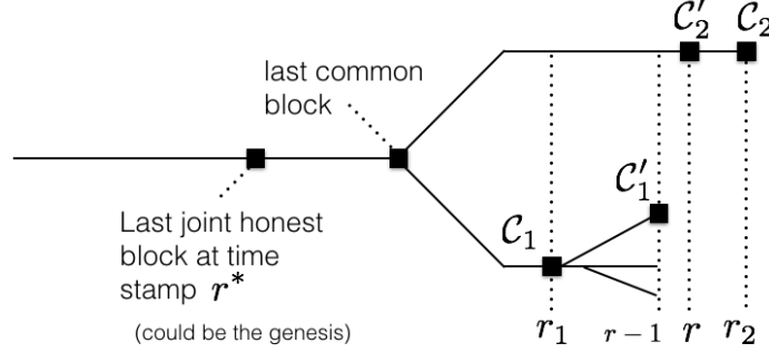
Figure 3: Chains from the proof of Theorem 15. Round r is the first round, where an honest party adopts a chain \mathcal{C}'_2 with \mathcal{C}'_1 \not\preceq \mathcal{C}'_2
