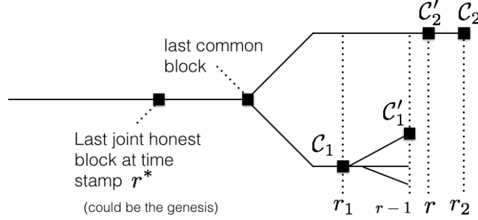
Figure 3: Chains from the proof of Theorem 15. Round r is the first round, where an honest party adopts a chain \mathcal{C}'_2 with \mathcal{C}_1^{\lceil k} \not\preceq \mathcal{C}'_2
