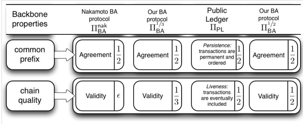
Figure 1: An overview of the backbone protocol’s applications: Nakamoto’s BA protocol \Pi_{BA}^{\text{nak}} , our BA protocols \Pi_{BA}^{1/3} and \Pi_{BA}^{1/2} , and the public ledger protocol \Pi_{PL} . All properties must be satisfied with overwhelming probability. In each box we state the name of the property as well as the maximum ratio of the adversarial hashing power that we can prove the protocol withstands (based on the corresponding backbone property). The value \epsilon stands for a negligible quantity.
