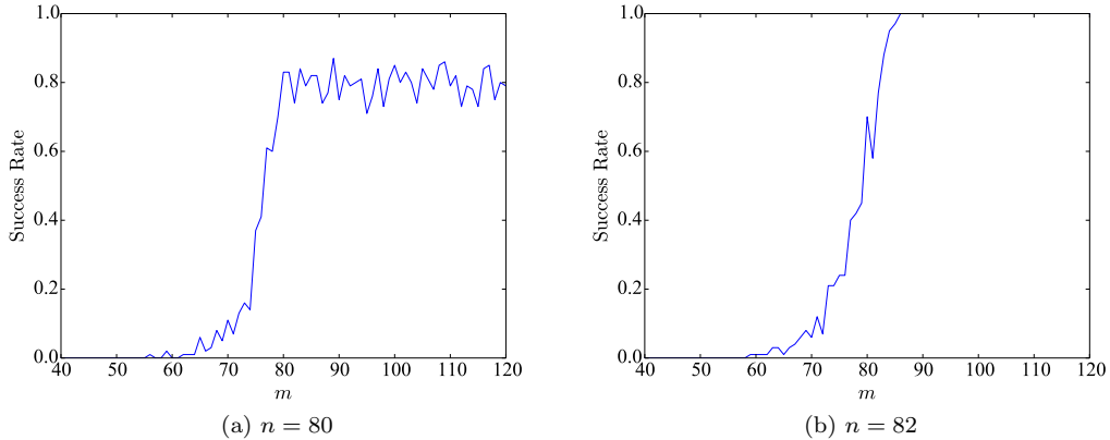
Figure 3: Success rate of finding \mathbf{x} from the system of linear congruences built from Eq. (3).
