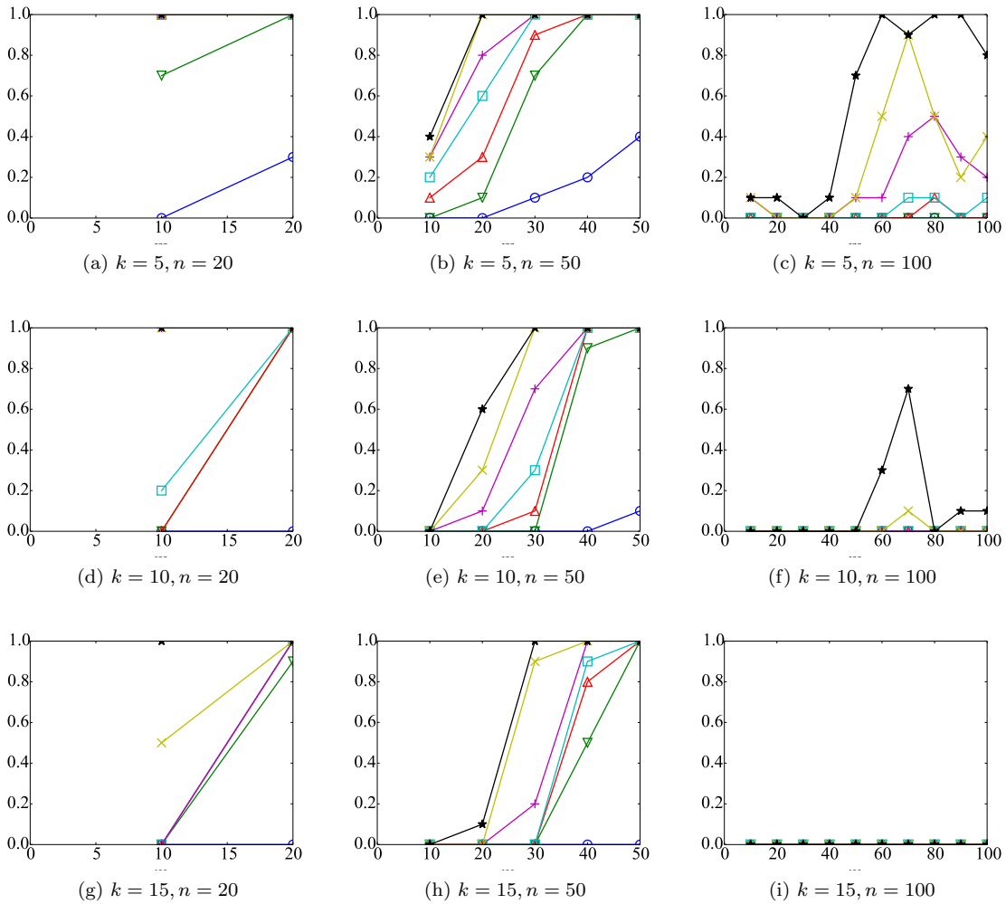
Figure 1: The success of the LLL algorithm against different values of d , k , m and n . The x -axis in the graphs represents m . The y -axis is the success percentage. Legend: \circ d=2 , \nabla d=3 , \triangle d=4 , \square d=5 , + d=7 , \times d=10 , \star d=15 .
