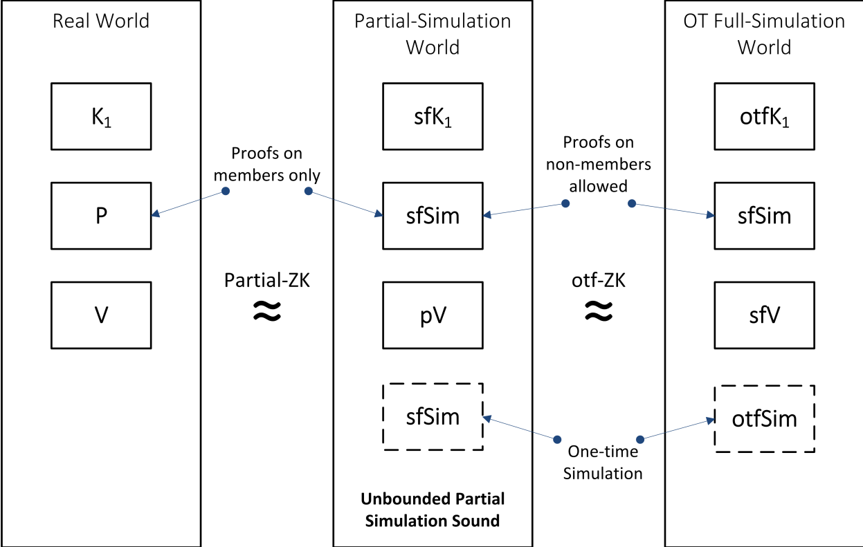
Figure 1: The three worlds of a DSS-QA-NIZK
