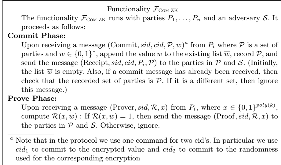
Fig. 2. Ideal functionality \mathcal{F}_{\text{COM-ZK}} .
