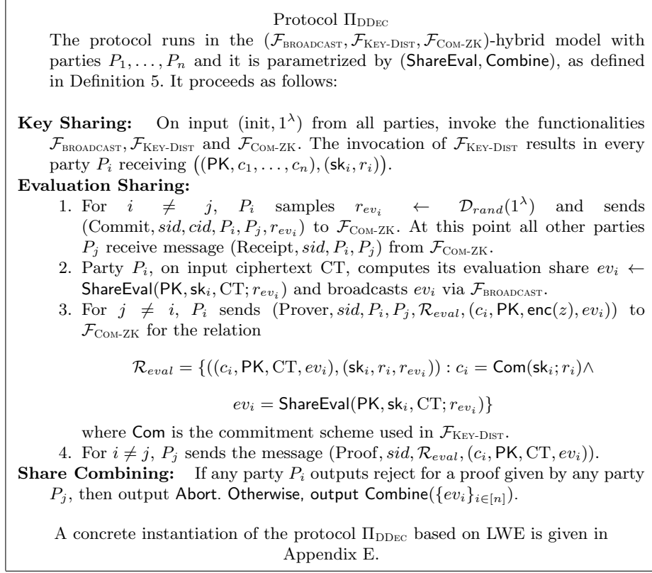
Fig. 6. Distributed decryption protocol.
