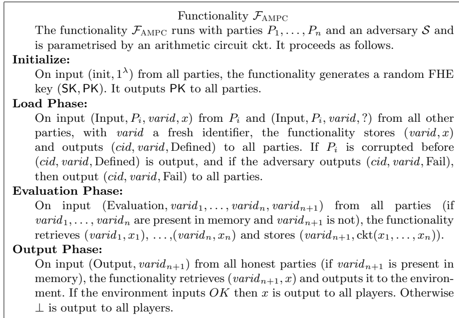
Fig. 5. Ideal functionality for Arithmetic MPC.
