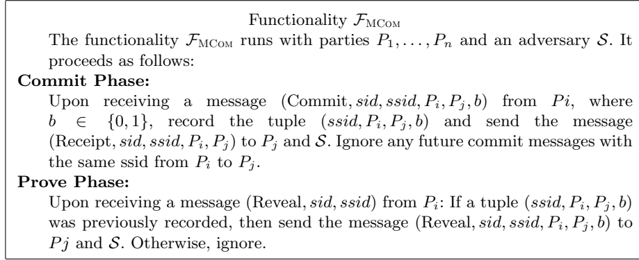
Fig. 8. The ideal functionality \mathcal{F}_{\text{MCOM}} .
