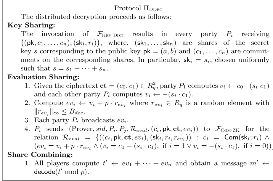
Fig. 7. The threshold decryption protocol.
