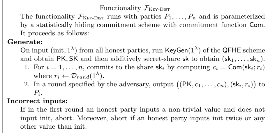
Fig. 4. Ideal functionality \mathcal{F}_{\text{KEY-DIST}} .
