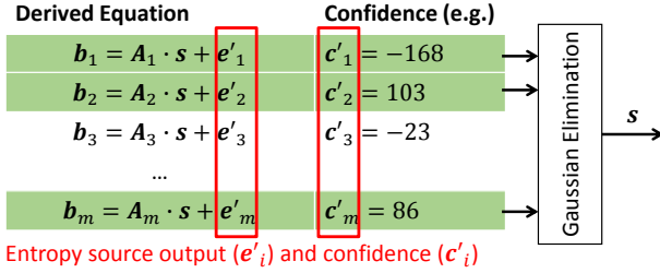
Fig. 2: Overview of LPN key extraction algorithm. The e'_i values are regenerated and the c'_i values with high absolute value identify the e'_i with low probability of error (since c'_i values don't change dramatically between measurements, and e'_i = \text{Sign}(c'_i) ). Gaussian elimination is then used on these selected equations to extract the secret key.
