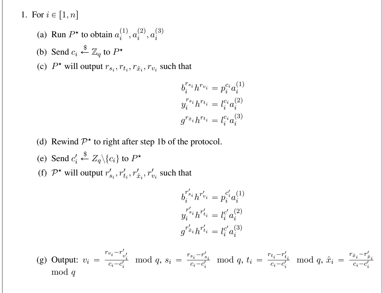
Figure 6: Extractor for Proof of Assets protocol
