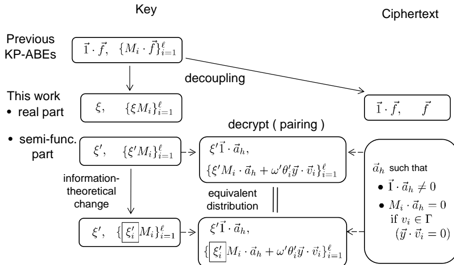
Fig. 1. Decoupling of LSS matrix from randomness and partial LSS randomization in semi-functional parts. Here, (M = (M_i), \rho) is an access structure, uniformly random \vec{f} \leftarrow^U \mathbb{F}_q^r , \xi, \xi', \xi'_i, \theta'_i \leftarrow^U \mathbb{F}_q , \vec{y} := (y_1, \dots, y_n) such that \sum_{j=0}^{n-1} y_{n-j} z^j = z^{n-1-n'} \prod_{j=1}^{n'} (z - x_j) , and \vec{v}_i := (v_i^{n-1}, \dots, v_i, 1) for v_i := \rho(i) .
