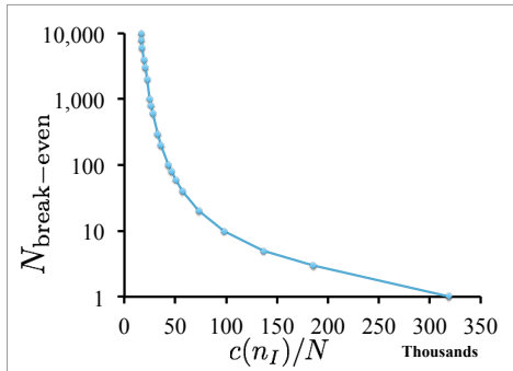
Fig. 10: Quantifying N_{\text{break-even}} with respect to c(n_I)/N , the cost ratio of input handling and circuit size.
