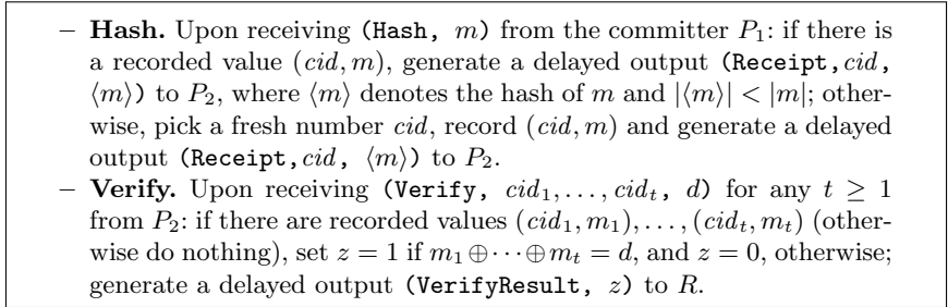
Fig. 2: Ideal functionality of XOR-Homomorphic Interactive Hash. (“send a delayed output x to party P ” signals a standard treatment of fairness: it means “send (x, P) to the adversary; when receiving ok from the adversary, output x to P .”)
