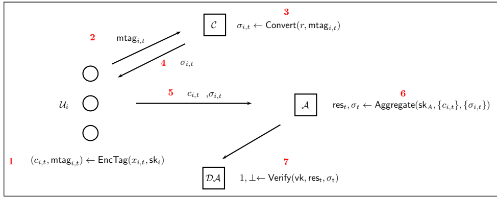
Figure 1: Basic idea for collusion resistant aggregation. Users encrypt their data with an additively homomorphic encryption scheme. They also tag their data at first layer with a metatag \text{mtag}_{i,t} at step 1. Afterwards, user U_i forwards it to the Converter C . C converts the metatag to the final tag \text{tag}_{i,t} and transmits it to U_i at step 4. U_i sends to A the ciphertext c_{i,t} along with the the \text{tag}_{i,t} . A decrypts and learns the result \text{sum}_t . Finally, A forwards to C the result \text{sum}_t and the proof \sigma_t that allows the data analyzer DA , who acts as a honest verifier, verify the correctness of computation performed by a malicious Aggregator A .
