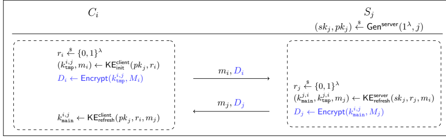
Fig. 2: Execution of a 0-RTT KE Protocol with Server-Only Authentication in Parallel to Encrypted Application Data. Note that the messages D_i and D_j correspond to the symmetric encryption protocol used to encrypt payload data, and are therefore not part of the 0-RTT KE protocol, but a separate protocol. These messages are only displayed here only to illustrate the basic, parallel application message flow to that of a 0-RTT KE protocol. While it would in principle be possible to define the symmetric encryption directly as part of the protocol, this would require a significantly more complex “ACCE-style” [16] security model, which we avoid for sake of simplicity.
