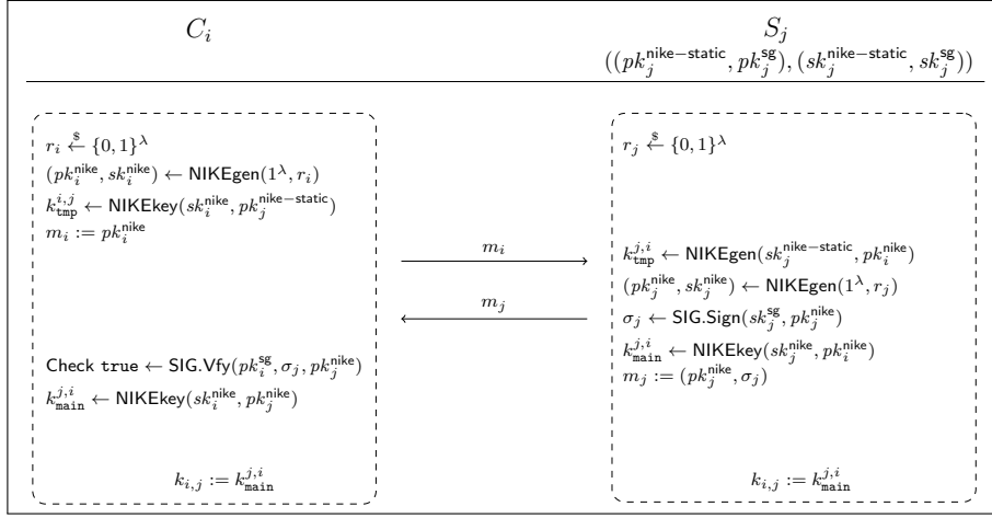
Fig. 3: 0-RTT KE from NIKE. Again, it is possible to include the parallel execution of a symmetric encryption protocol which would behave as in Figure 2 for encrypted application data. As such a protocol is not part of the 0-RTT KE protocol, we omit it here for simplicity.
