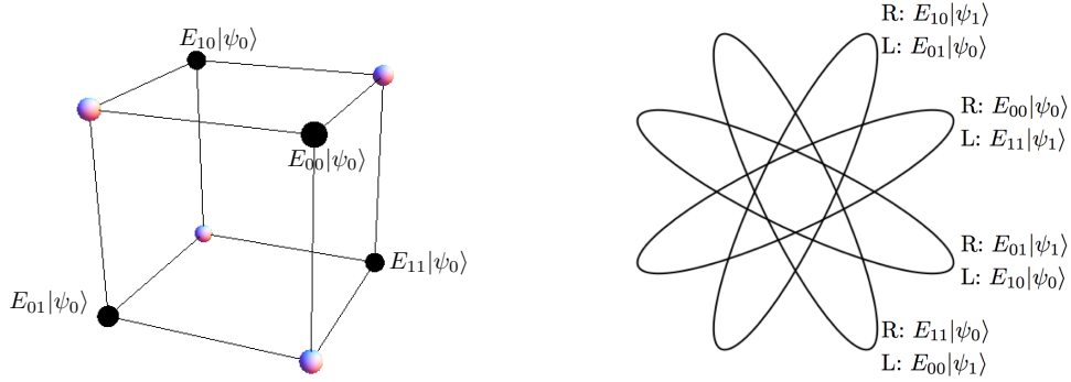
Figure 2: The eight cipherstates |\psi_{uwg}\rangle = E_{uw}|\psi_g\rangle shown (left) on the Bloch sphere, forming the corner points (\pm 1, \pm 1, \pm 1)/\sqrt{3} of a cube; and (right) as elliptic polarisation states. ‘R’ stands for righthanded, ‘L’ for lefthanded.
