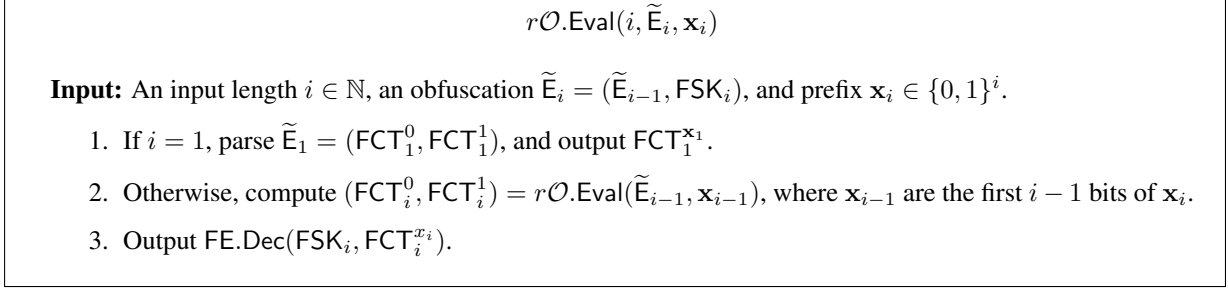
Figure 2: The recursive evaluation procedure.
