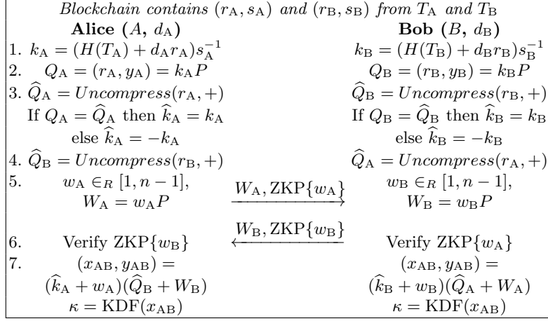
Fig. 3. YAK-over-Bitcoin Protocol
