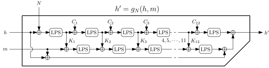
Fig. 2. Streebog compression function. All data paths, inputs, and outputs are 512-bit vectors. Here the \oplus symbol denotes the XOR operation between two 512-bit vectors.
