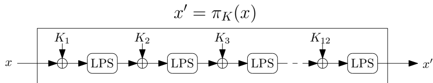
Fig. 3. The 512-bit permutation \pi used by StriBob.
