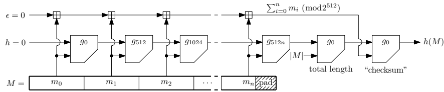
Fig. 1. Operation of Streebog with 512-bit output. For 256-bit hashes, the initial h value is changed to 0 \times 01010101 \dots 01 and the output h(M) is truncated to 256 bits.
