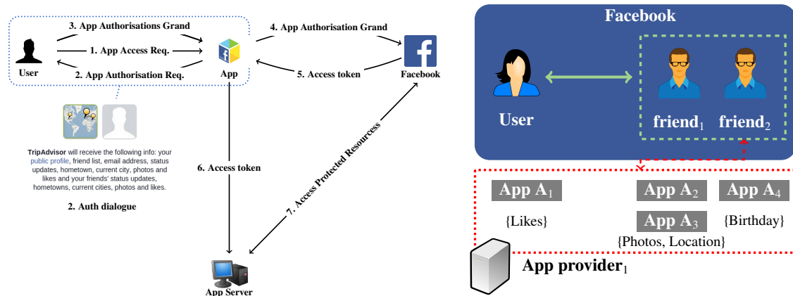
Fig. 1. (a) Facebook Developers app architecture, (b) Collateral information collection scheme on Facebook
