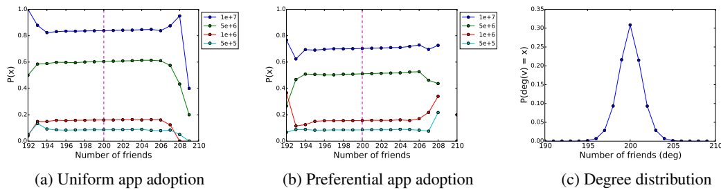
Fig. 10. Simulation results on a WS graph with k = 1,000,000 and d = 200 .
