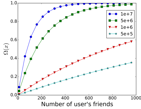
Fig. 7. Likelihood of collateral information collection based on real data [9] (per MAU).
