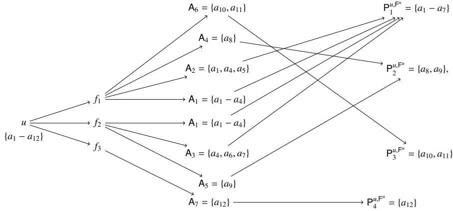
Fig. 11. Example for collateral information collection while enabling profiling to P_j .
