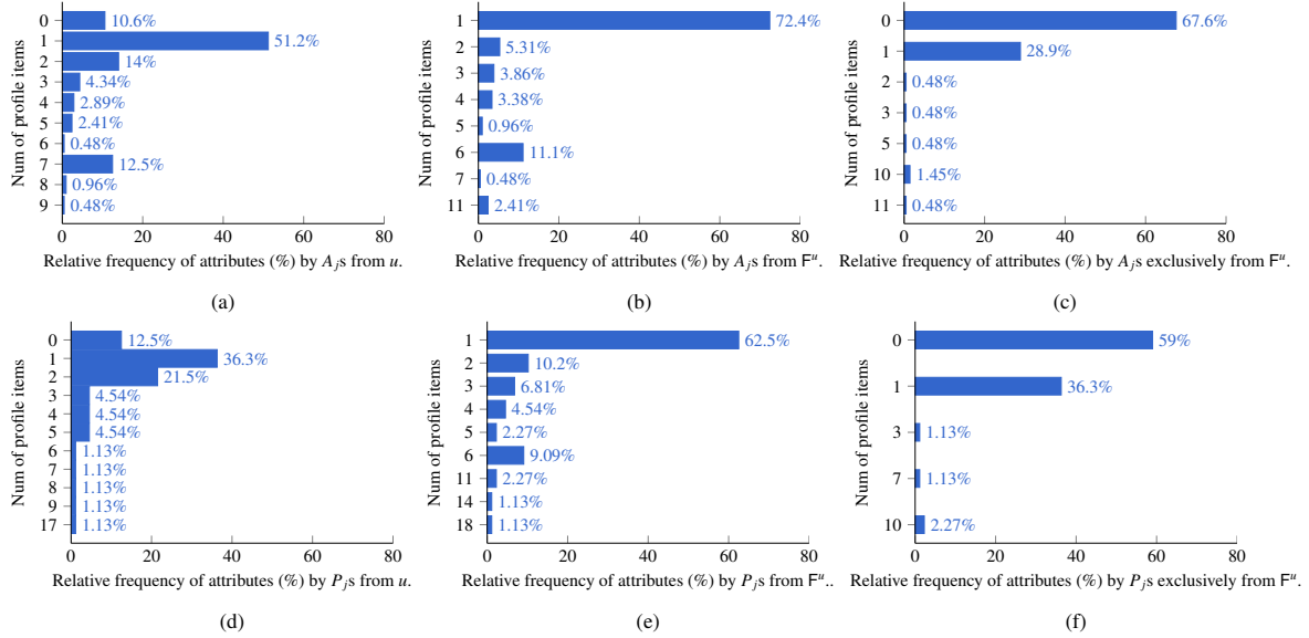
Fig. 14. Number of attributes gathered via direct, collateral and exclusive Collateral Information Collection wrt apps ( A_j , top) and app providers ( P_j , bottom)
