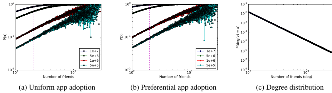
Fig. 9. Simulation results on a BA graph with k = 1,000,000 and d = 200 .
