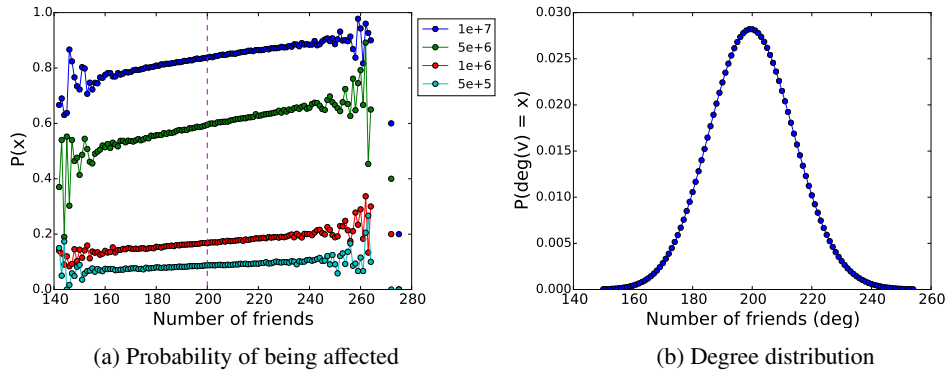
Fig. 8. Simulation results on an ER graph with k = 1,000,000 and d = 200 .
