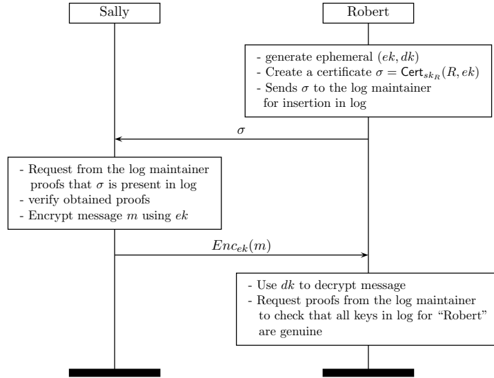
Figure 2: The basic DECIM protocol. Robert has a pair (sk_R, vk_R) of long term keys for signature signing and verification. He generates an ephemeral key pair (ek, dk) for encryption, creates the certificate \sigma = \text{Cert}_{sk_R}(R, ek) on ek , and sends the certificate to the log maintainer for insertion into the public log. Meanwhile, Robert also sends the certificate to Sally. After receiving \sigma , Sally requests from the log maintainer proofs that the certificate is present in the log. If the proof is valid, Sally sends a message m to Robert encrypted with ek . Robert requests proofs from the log maintainer to enable him to verify whether the log contains signatures that he did not generate.
