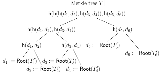
Figure 4: An example of the log containing six updates \{d_1, d_2, \dots, d_6\} . The log is an append-only Merkle tree T whose leaves are ordered chronologically.
