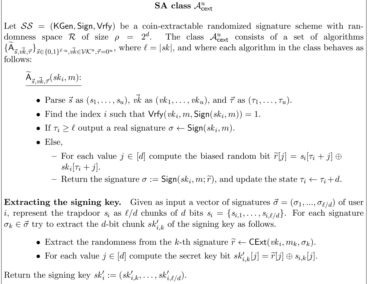
Figure 7: Attacking coin-extractable schemes in the multi-user setting
