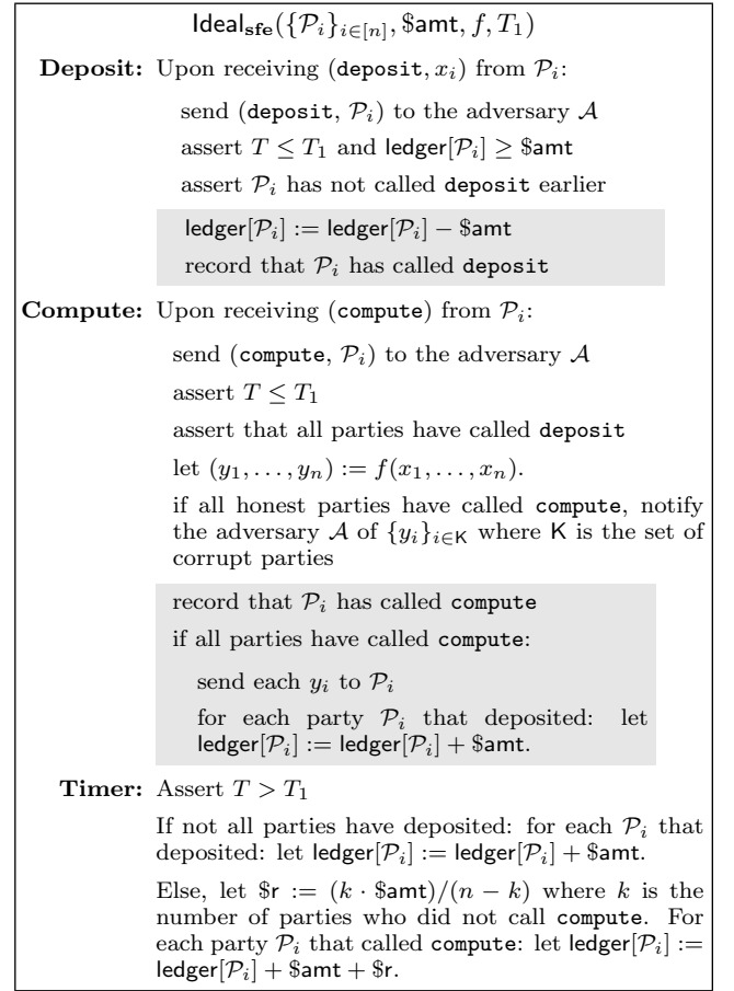
Figure 15: Ideal program for fair secure function evaluation.
