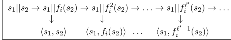
Figure 5: One iteration of BM-PRG
