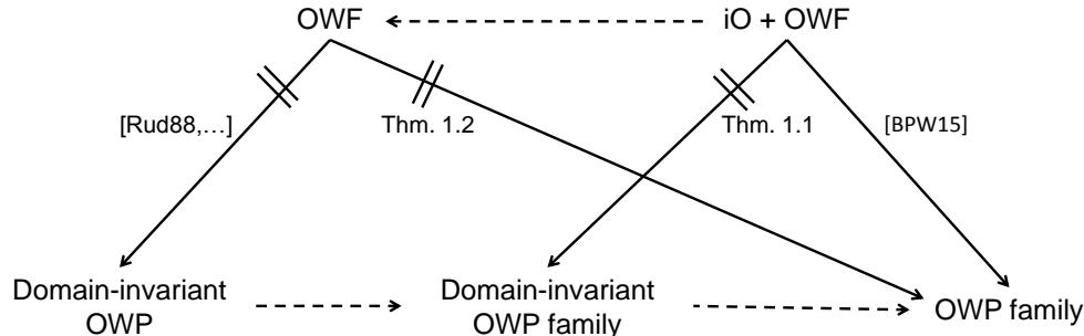
Figure 1: A dashed arrow from a primitive A to a primitive B indicates that A implies B by definition. Bitansky et al. [BPW15] showed that any sub-exponentially-secure indistinguishability obfuscator and one-way function imply a one-way permutation family (which is not domain invariant), and we show that one cannot construct the stronger primitive of a domain-invariant one-way permutation family unless new non-black-box techniques are introduced (even when assuming sub-exponential security). The line of research starting with Rudich [Rud88] showed that one cannot construct a domain-invariant one-way permutation from a one-way function in a black-box manner. We improve this result, showing that one cannot construct the weaker primitive of a one-way permutation family (even one that is not domain invariant) from a one-way function in a black-box manner (again, even when assuming sub-exponential security).
