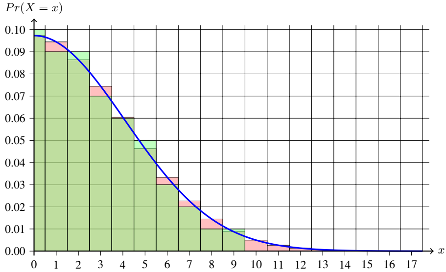
Fig. 3. Sampling the discrete Gaussian distribution with \sigma = 4.1 and sampling precision 0.01. The red (rounded down) and green (rounded up) area illustrates the statistical distance (total variation distance) \epsilon between the ideal distribution and sampling with the precision of the grid. Only the positive half x > 0 of the symmetric distribution is shown. All |x| \geq 10 are “tail”.
