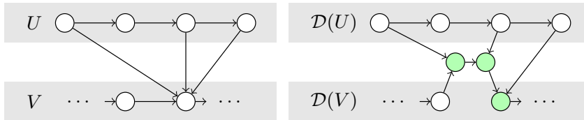
Fig. 10: A portion of a sandwich graph G (left) and the same portion of the corresponding degree-reduced graph \mathcal{D}(G) (right). The shaded vertices are part of the degree-reduction gadget.
