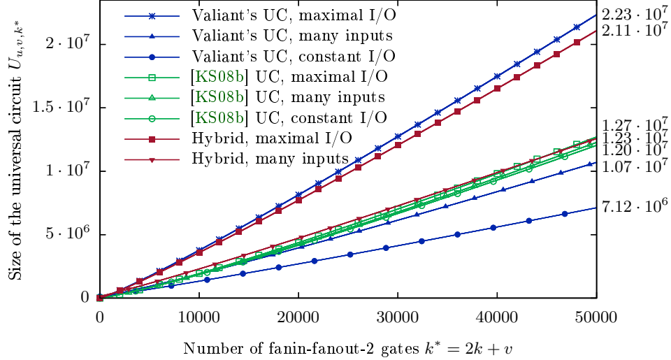
Fig. 9: Comparison between the sizes of the UC constructions for k^* = 2k + v \in \{0, \dots, 50\,000\} gates, considering the three scenarios: constant I/O with constant number of inputs and outputs, many inputs with \sim k inputs and constant outputs and maximal I/O with \sim 2k inputs and \sim k outputs.
