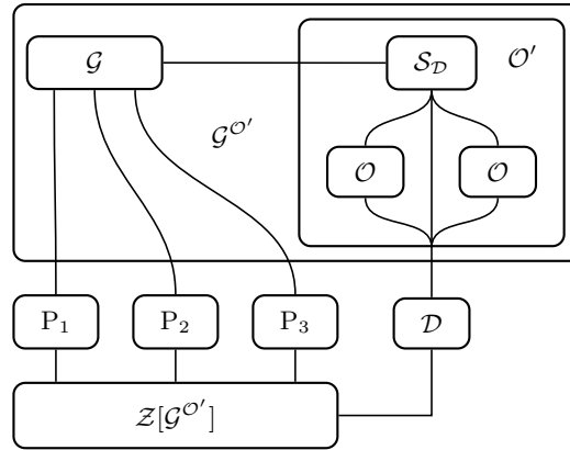
Fig. 6. The functionality \mathcal{G} with composed oracle \mathcal{O}'
