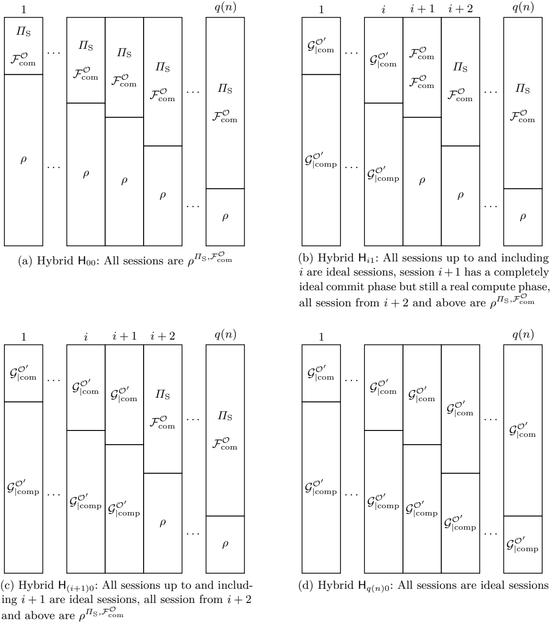
Fig. 7. The sequence of hybrids H_{ib} (see proof of Theorem 26): The notation \mathcal{G}'_{\text{comp}}^O denotes the “compute phase” of an ideal \mathcal{G} -session and \mathcal{G}'_{\text{com}}^O denotes the “commit phase” of an ideal \mathcal{G} -session
