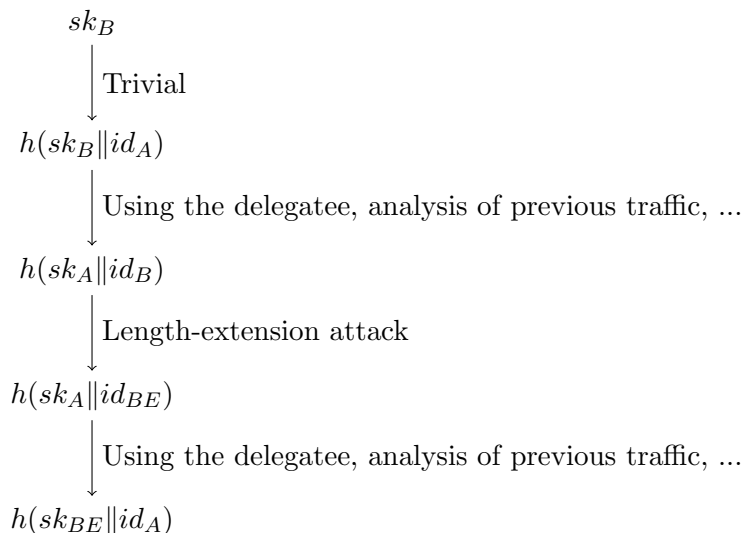
Figure 6: Abstract flow of a length-extension attack
