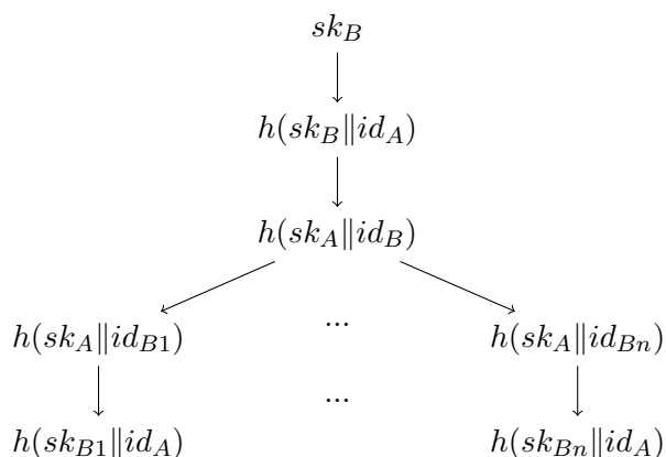
Figure 7: Abstract flow of a sybil attack
