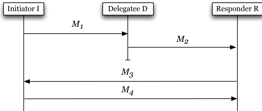
Figure 2: Protocol flow
