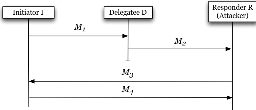
Figure 5: Flow of the KCI Attack 3
