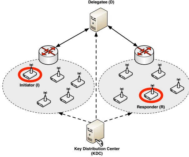
Figure 1: Network architecture (adapted from [22])
