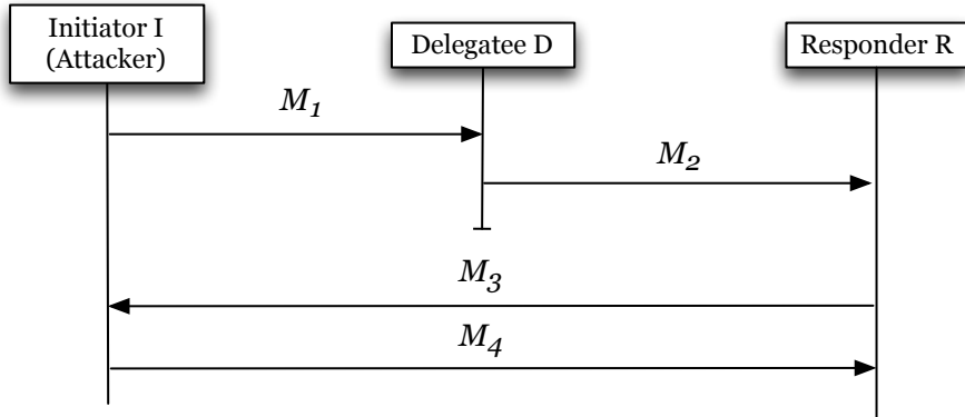
Figure 4: Flow of the KCI Attack 2
