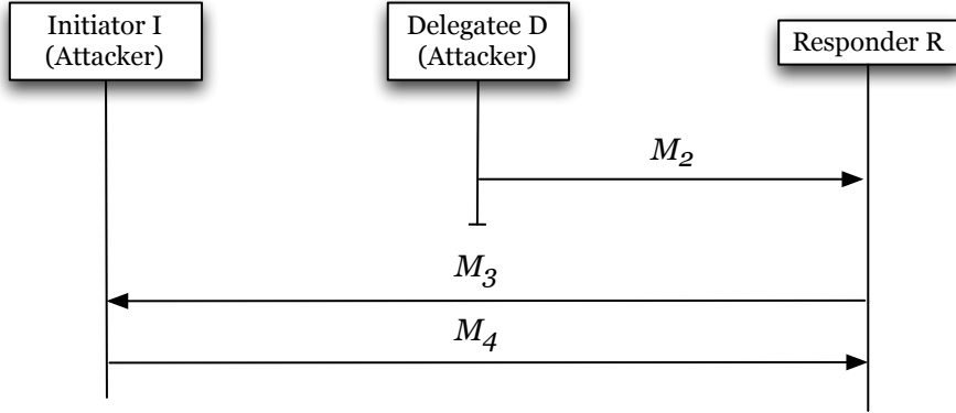
Figure 3: Flow of the KCI Attack 1
