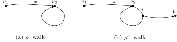
Fig. 2: The graphs corresponding to \rho and \rho' walks. Note that the lengths of the parts labeled with * can be zero.
