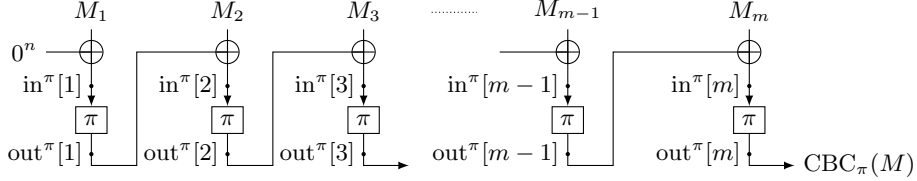
Fig. 3: CBC function and its intermediate values.
