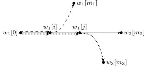
Fig. 7: Free structure graph for three messages.
