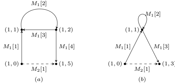
Fig. 6: The counter examples. (a) M_1 = (M_1[1], M_1[2], M_1[3], M_1[2], M_1[4]) and M_2 = (M_2[1]) be two messages such that M_2[1] := M_1[1] \oplus M_1[3] \oplus M_1[4] . Here we have two input-collisions \delta_1 := ((1, 0), (1, 2) ; (1, 1)) and \delta_2 := ((1, 0), (1, 2) ; (1, 5)) . The two linear equations L_{\delta_1} and L_{\delta_2} corresponding to the two input-collisions are same as Y_{(1,0)} \oplus Y_{(1,2)} = M_1[1] \oplus M_1[3] and so the rank (which is also the accident in this case) is one. However, true collision is two (at (1, 1) and (1, 5) ) which contradicts [3, Lemma 10]. Similar arguments can be given for figure (b), where M_1 = (M_1[1], M_1[2], M_1[3]) and M_2 = (M_2[1]) , such that M_2[1] := M_1[1] \oplus M_1[2] \oplus M_1[3] .
