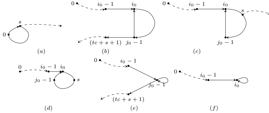
Fig. 8: Characterizing all accident-one structure graphs realizable by a single message. The dashed lines in these illustrations represent optional subwalks. Here the vertex w[i] is represented by i , for notational simplicity.
