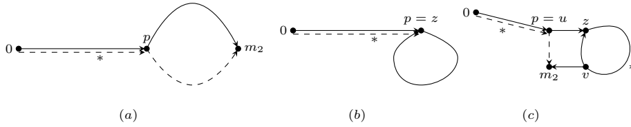
Fig. 9: Characterizing all accident-one structure graphs realizable by two messages which satisfy the \text{coll} event. Dashed lines represent w_1 and solid lines represent w_2 .
