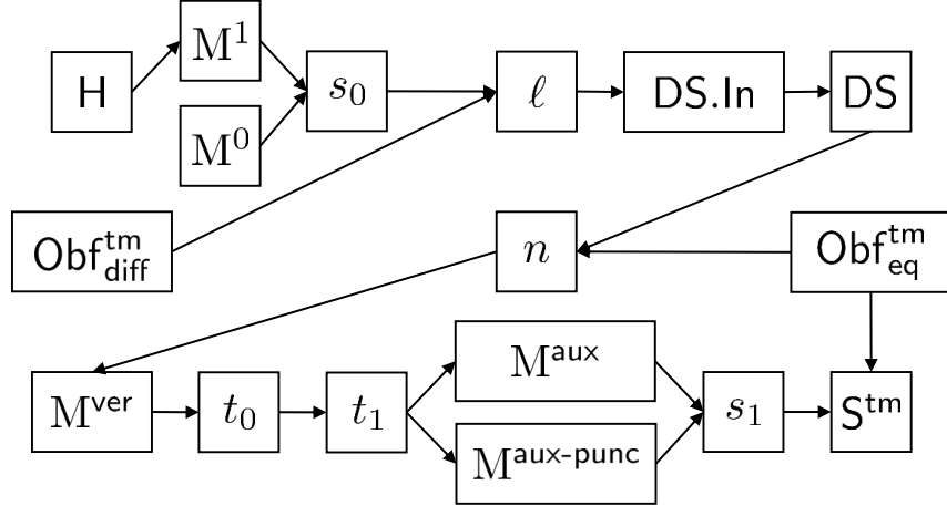
Figure 7: Parameter dependencies in TM-SAMP for the proof of Theorem 4.1.
