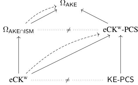
Figure 5: Relationship between the various models we define in this section. \Omega_{AKE\cap ISM} and eCK^w are from [14] and [15] respectively. We propose the other three modules in this work. Solid arrows denote inequality of security models ( \leq_{sec} , Appendix B), dotted arrows denote incomparability (neither model implies the other), and dashed arrows denote our transformation. For example, in this set \Omega_{AKE} provides the strongest security guarantees.
