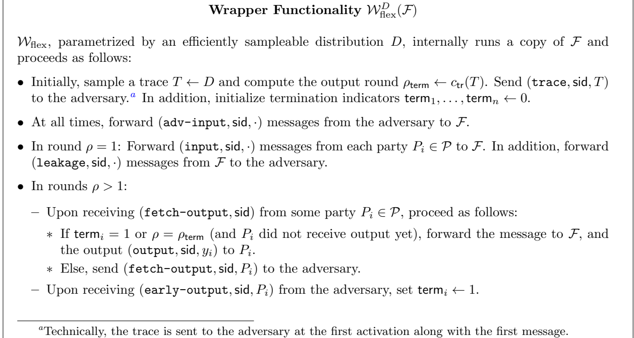
Figure 5: The flexible-wrapper functionality
