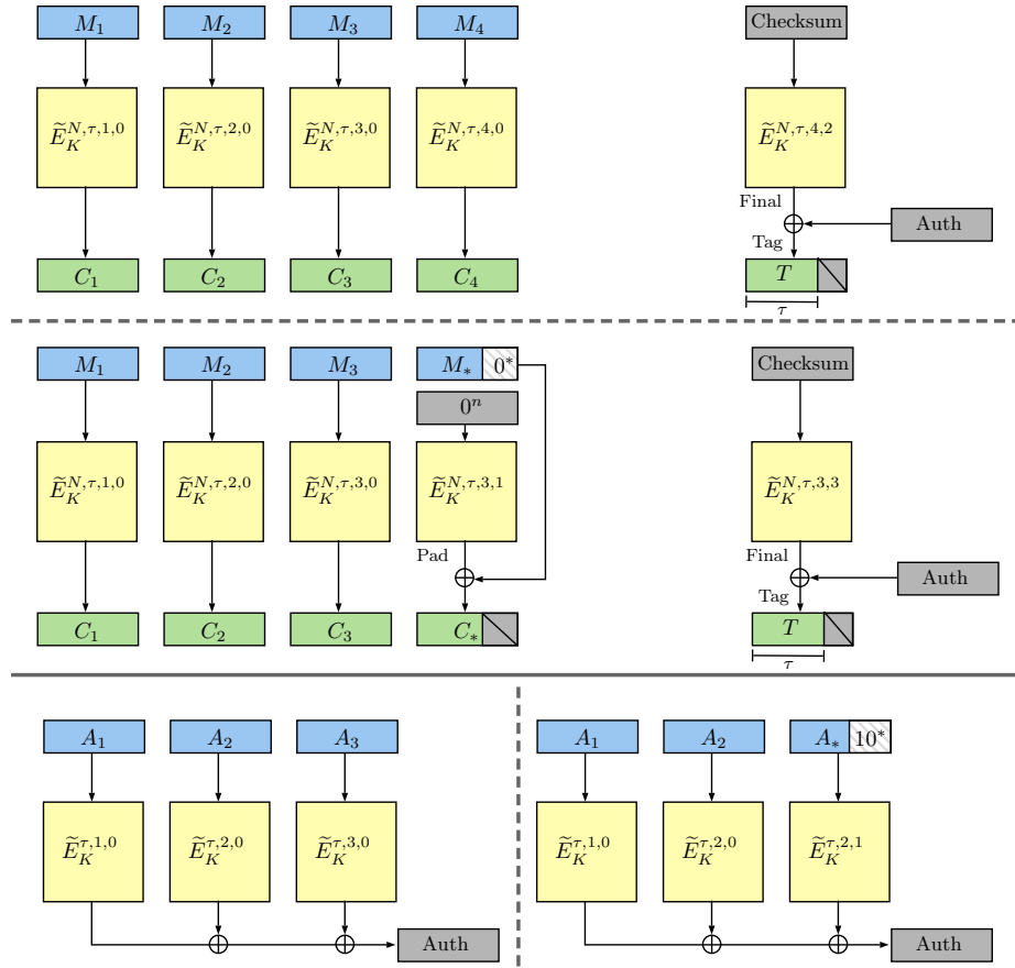
Fig. 16: Illustration of the encryption process of \Theta\text{CBv} (inspired by [?]) instantiated with a tweakable blockcipher \tilde{E} : \mathcal{K} \times \mathcal{T} \times \{0, 1\}^n \rightarrow \{0, 1\}^n . The top half depicts the encryption of a message with four complete blocks (top) with \text{Sum} = \bigoplus_{i=1}^4 M_i and the encryption of a message with three complete blocks and an incomplete block (bottom) with \text{Sum} = \bigoplus_{i=1}^3 \oplus M_* || 10^n . The bottom half of the picture shows processing of associated data of three complete blocks (left) or two complete blocks and an incomplete block (right).
