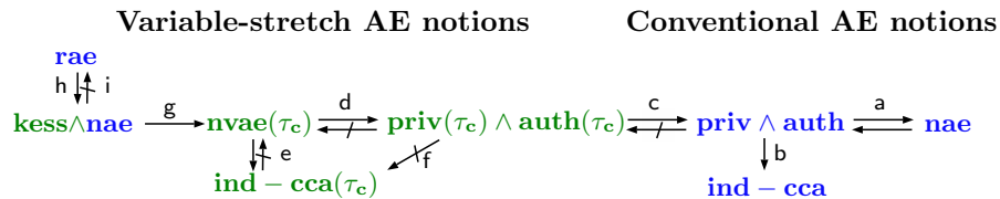
Fig. 1: Relations among notions for nonce-based AE with and without variable stretch. Previous works: a [?], b [?]. This paper: c (Remark ??, attacks in Section ??), d (Remark ??, Corollary ??), e (Theorem ??, Remark ??), f (Proposition ??), g (Theorem ??), h, i (Remark ?? together with [?]).
