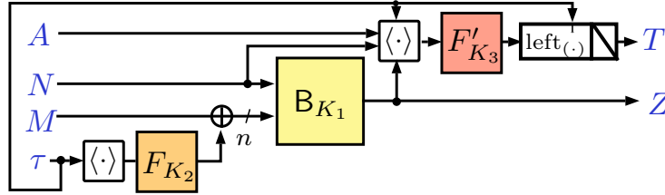
Fig. 10: The encryption algorithm of the scheme \Pi\text{-cca} . \langle \cdot \rangle is an efficiently computable, injective encoding scheme.
