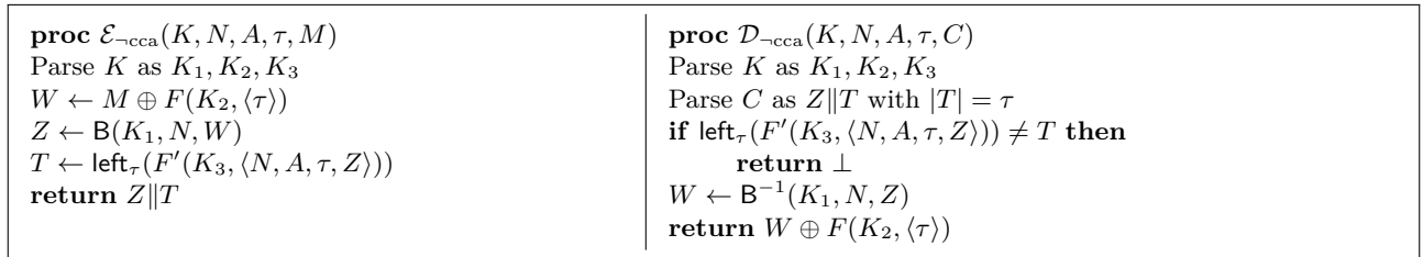
Fig. 11: Encryption and decryption algorithms of the nonce-based, variable-stretch AE scheme \Pi\text{-cca} = (\mathcal{K}\text{-cca}, \mathcal{E}\text{-cca}, \mathcal{D}\text{-cca}) . \langle \cdot \rangle is an efficiently computable, injective encoding scheme.
