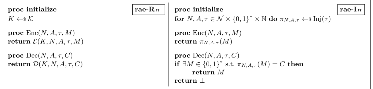
Fig. 4: RAE security . Defining security for a robust AE scheme \Pi = (\mathcal{K}, \mathcal{E}, \mathcal{D}) with nonce space \mathcal{N} . \text{Inj}(\tau) denotes the set of all injective, \tau -expanding functions from \{0, 1\}^* to \{0, 1\}^{\geq \tau} .
