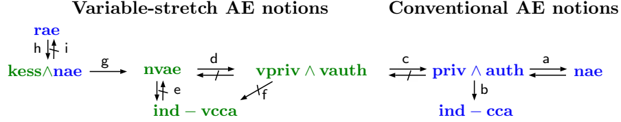
Fig. 1: Relations among notions for nonce-based AE with and without variable stretch. Previous works: a [36], b [3]. This paper: c (Remark 3, attacks in Section 3), d (Remark 3, Corollary 1), e (Theorem 1, Remark 2), f (Proposition 1), g (Theorem 2), h, i (Remark 4 together with [16]).
