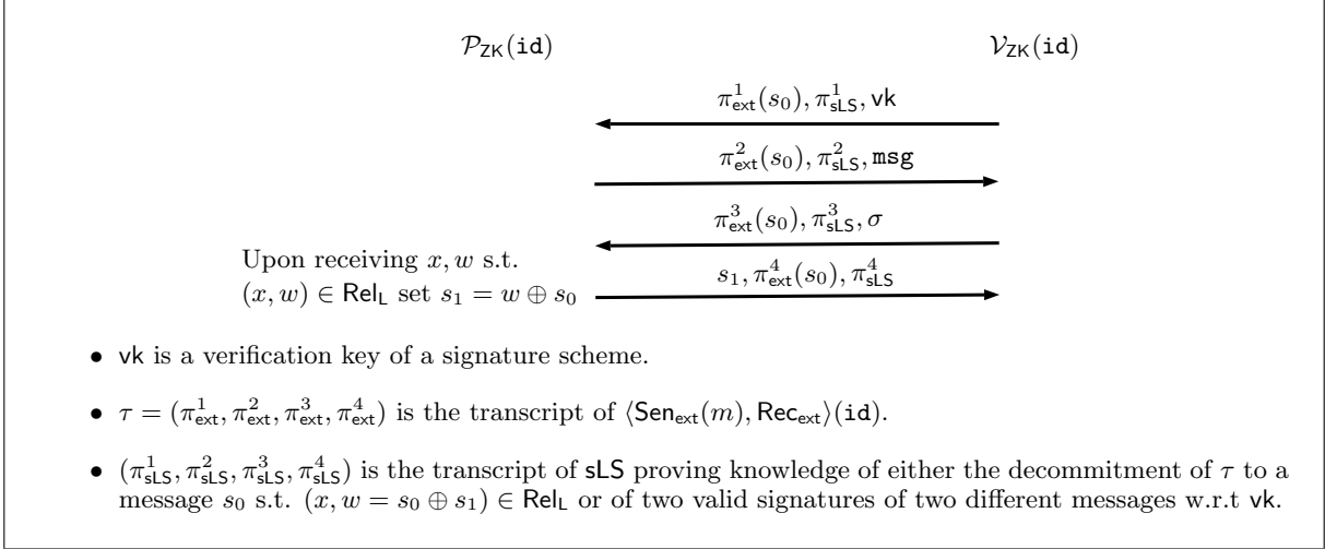
Figure 3: Informal description of our delayed-input 4-round NMZK AoK \Pi_{\text{ZK}} .
