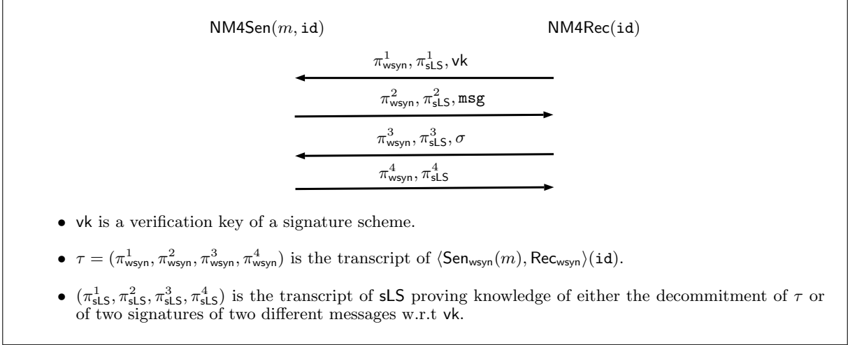
Figure 1: Informal description of our 4-round NM commitment scheme \Pi_{\text{NM4Com}} .
