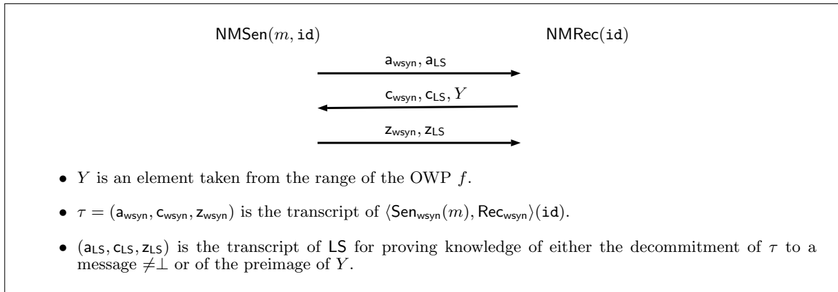
Figure 5: Informal description of our 3-round NM commitment scheme \Pi_{\text{NMCom}} .
