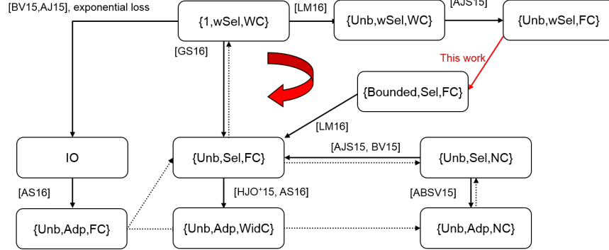
Figure 1: The state-of-art relationships between different notions of IND-FE scheme. This work is given by the red arrow and the alternative approach is given by the bold red arrow. Non-trivial relationships are given by solid arrows and trivial relationships are given by dotted arrows.
