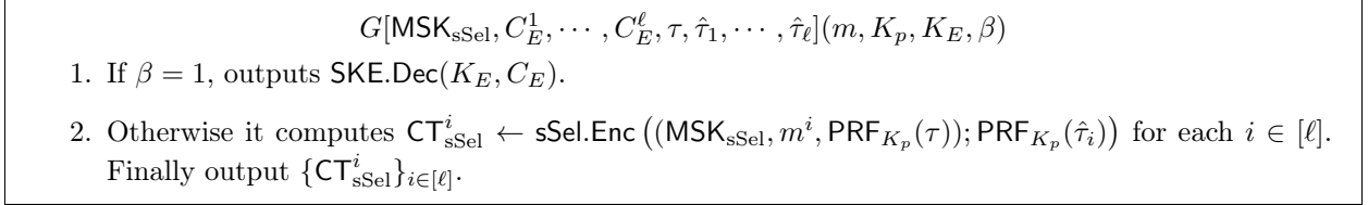
Figure 2: The circuit G[\text{MSK}_{\text{sSel}}, C_E^1, \dots, C_E^\ell, \tau, \hat{\tau}_1, \dots, \hat{\tau}_\ell]
