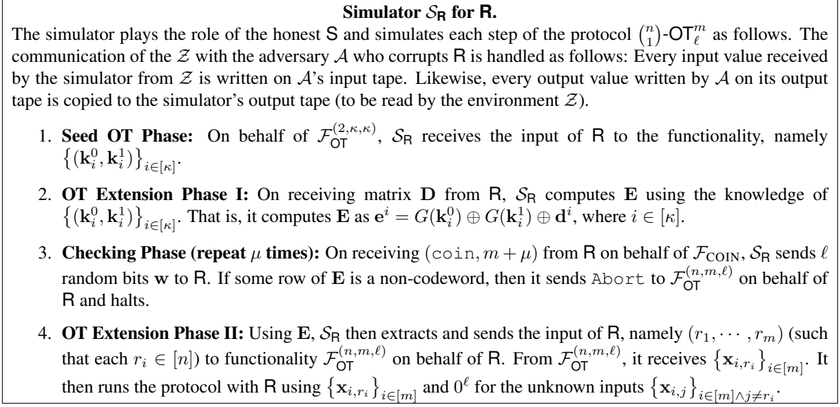
Figure 7: Simulator \mathcal{S}_R for Malicious Receiver
