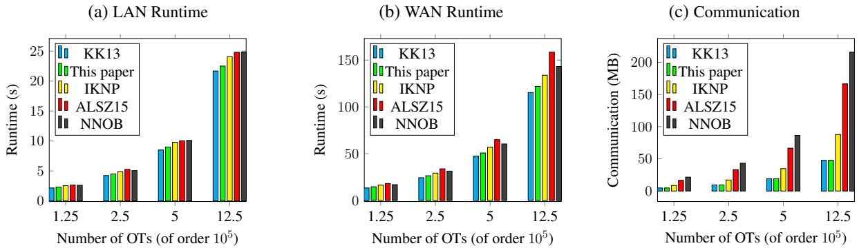
Figure 8: Performance Comparison of various OT extensions for producing \binom{16}{1} -OT _4^m .
