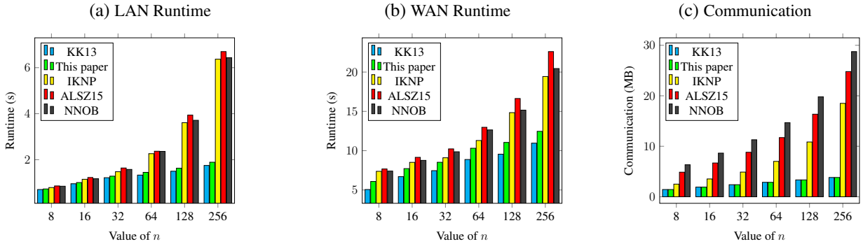
Figure 9: Performance Comparison of various OT extensions for producing \binom{n}{1} -OT _{\log n}^{5 \times 10^4} .
