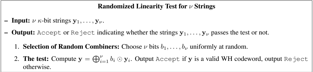
Figure 2: A Randomized Linearity Test for Many Strings
