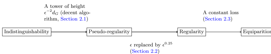
Fig. 1. An overview of our proof of the Strong Regularity Lemma.
