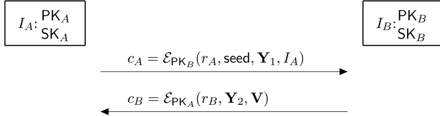
Figure 19: Basic Structure of CNKE from OKCN/AKCN-MLWE
