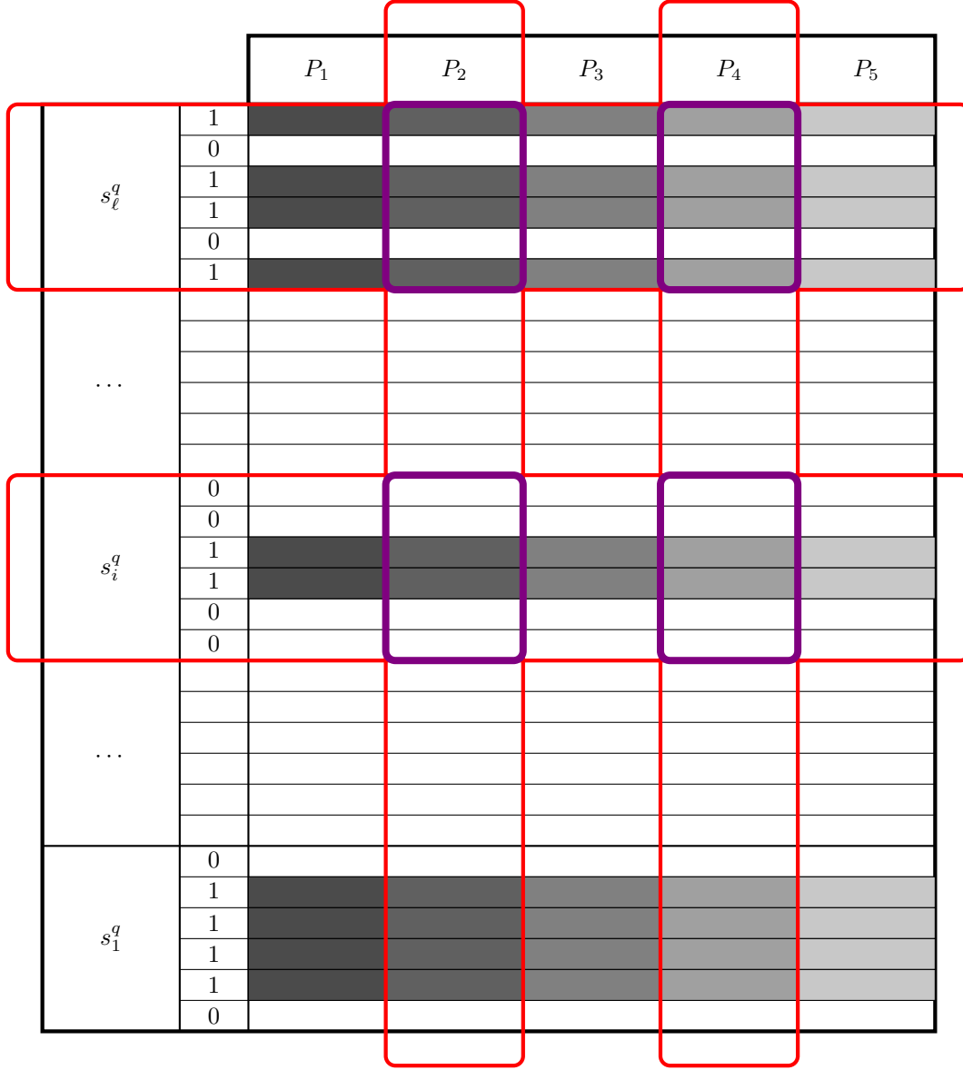
Fig. 17. A pictorial representation of the Prover's output in the NI Simulatable Proof System II. Let \ell = 5 be the number of parties, and \lambda be the security parameter. In the q -th iteration, each party P_i for i \in [\ell] has inputs (w_i^q, s_i^q) . We encode each s_i^q as s_i^q || \bar{s}_i^q , where \bar{s}_i^q is the bit-wise complement of s_i^q . For example 001 is encoded as 001100. For each bit of the encoding of s_i^q , if the bit is 1 then each party P_i places a weak encryption of its view, \text{view}_i , in the corresponding slot (represented by filled-in rectangles of various shades of gray in the figure). Otherwise, if the bit is 0 then each party places a weak encryption of all 0's in the corresponding slot, (represented by blank rectangles in the figure). During verification, the verifier checks in the first step that input s = s_1^q \oplus s_2^q \oplus \dots \oplus s_\ell^q . To check the consistency of the views, the verifier selects 2 columns ( P_2 and P_4 ) and 2 rows ( s_i^q and s_\ell^q ) at random and does the following: (1) checks that s_i^q and s_\ell^q are consistent with the values read in the first step (2) runs Rec on the weakly encrypted views and checks that the resulting views are consistent with each other and internally.
