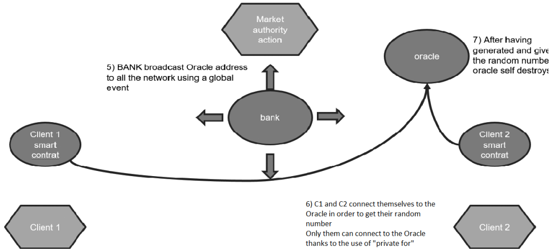
Figure 4: Random Number Generation
