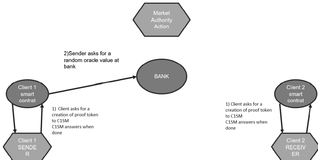
Figure 2: Proof Token Generation
