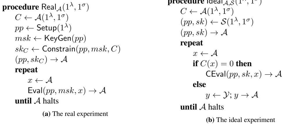
Figure 2: The real and ideal experiments.
