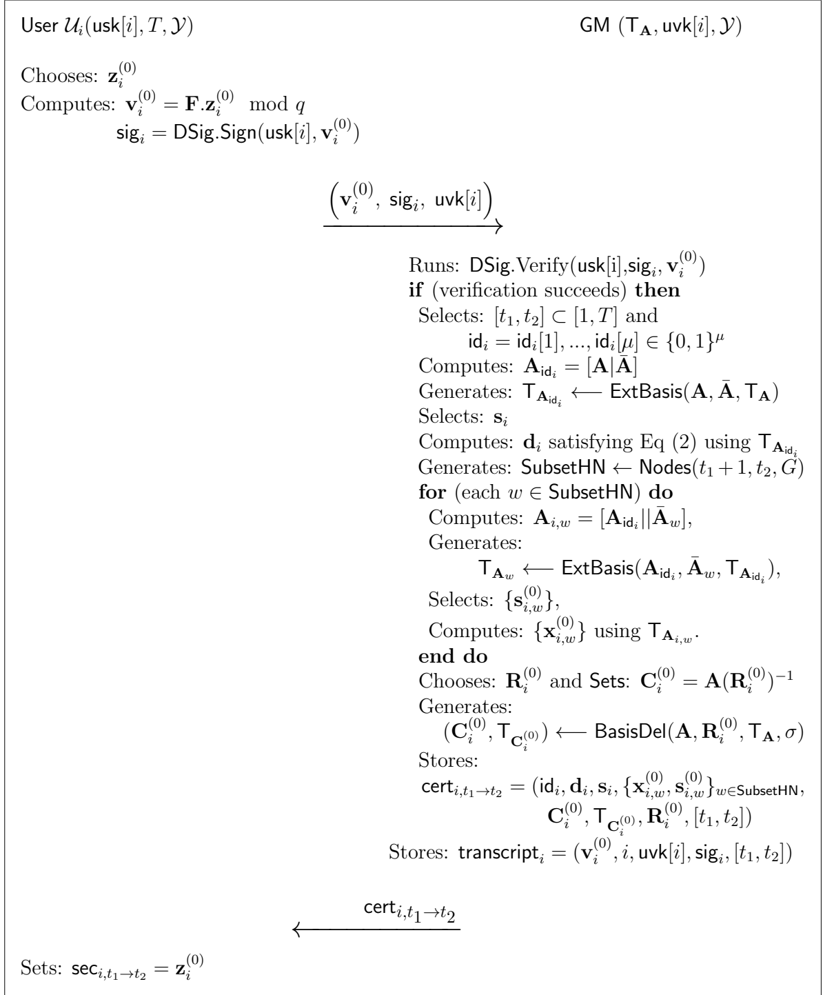
Figure 3: Join Algorithm
