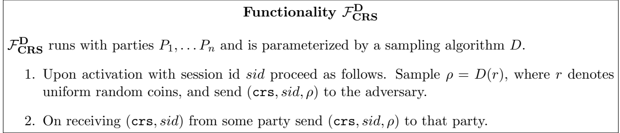
Figure 4: The Common Reference String Functionality.
