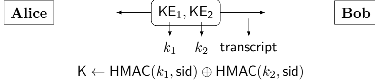
Figure 5: Hybrid protocol \Pi from authenticated key exchange protocols \text{KE}_1 and \text{KE}_2 .
