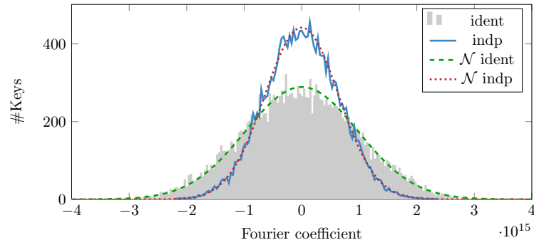
Distribution of Fourier coefficient for PRESENT with R_{19} and 10 rounds.
