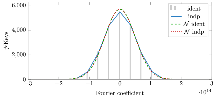
Distribution of Fourier coefficient for PRESENT with R_8 and 10 rounds.
