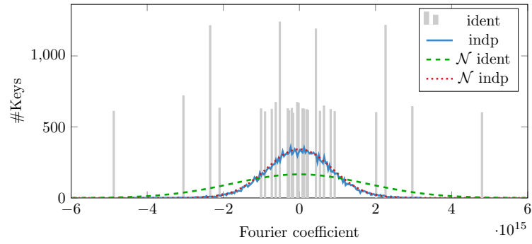
Distribution of Fourier coefficient for PRESENT with R_2 and 10 rounds.
