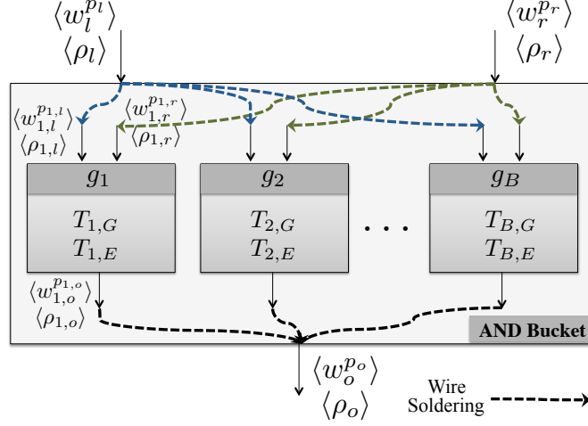
Fig. 5: A bucket of B garbled gates. (Wire labels and hashes exist at both the bucket-level (e.g. w_l^{p_l} ) and gate-level (e.g. w_{i,l}^{p_{i,l}} .)
