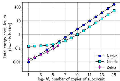
FIGURE 8—Energy cost of Giraffe, native baseline (§8.1), and Zebra [82, §8.2] versus number of copies of Curve25519 subcircuit. Each subcircuit computes 20 parallel evaluations of five sequential double-and-add steps. Untrusted technology node = 350 nm; trusted technology node = 7 nm; A_{\max} = 200 \text{ mm}^2 ; P_{\max} = 150 \text{ W} . Zebra’s scaling is limited to about 1150 parallel evaluations. Giraffe scales to more than 500× more parallel computations for the same chip area. Because of Giraffe’s refinements (§3), its improvement versus native is greater than Zebra’s. But Giraffe must amortize precomputation, while Zebra assumes it is free; thus, Giraffe needs larger N to break even.
