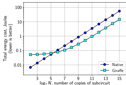
FIGURE 9—Energy cost of Giraffe and native baseline (§8.2) versus number of parallel image pyramid matching evaluations. Each evaluation matches 16-word needles against 128-word haystacks for a two-level image pyramid (§8.2). Words are represented as elements in \mathbb{F}_p , p = 2^{61} + 2^{19} + 1 . Untrusted technology node = 350 nm; trusted technology node = 7 nm; A_{\max} = 200 \text{ mm}^2 , P_{\max} = 150 \text{ W} . Giraffe breaks even for \approx 30 parallel searches.
