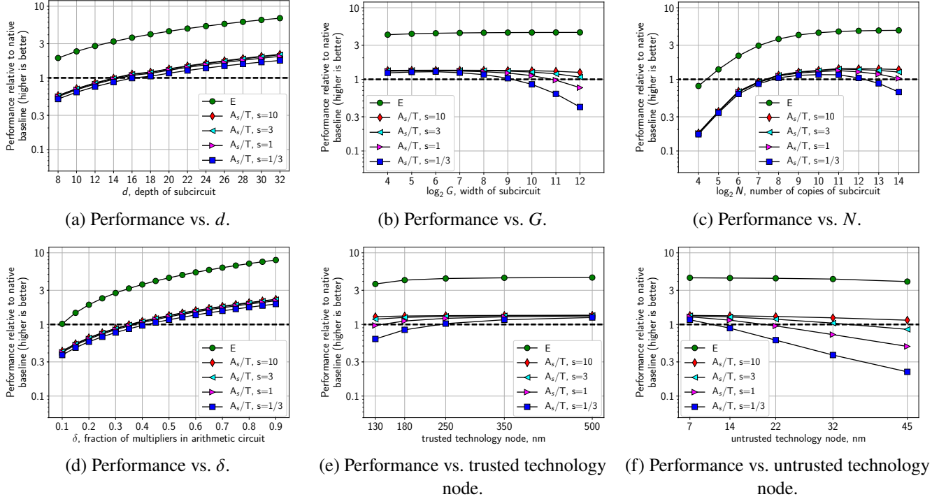
FIGURE 6—Giraffe’s overall performance ( \mathcal{V} and \mathcal{P} costs) compared to native baseline on E and A_s/T metrics (§6.2), varying AC parameters and technology nodes. In each case, we vary one parameter and fix the rest. Fixed parameters are: depth of \mathcal{C} , d = 20 ; width of subcircuit G = 2^8 ; number of sub-AC copies N = 2^{10} ; fraction of multipliers \delta = 0.5 ; trusted technology node = 350 nm; untrusted technology node = 7 nm; maximum chip area A_{\max} = 200 \text{ mm}^2 ; maximum power dissipation P_{\max} = 150 \text{ W} .
