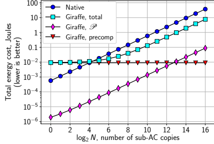
FIGURE 5—Evaluation of Giraffe’s back-end. We compare Giraffe’s costs to the native baseline, varying N . Giraffe beats native for N \approx 30 . Fixed AC parameters are: depth d = 20 ; width of sub-AC G = 2^8 ; fraction of multipliers \delta = 0.5 ; trusted technology = 350 nm; untrusted technology = 7 nm; maximum chip area A_{\max} = 200 \text{ mm}^2 ; maximum power dissipation P_{\max} = 150 \text{ W} . Per-gate energy costs for trusted and untrusted nodes are the same as in prior work [82, Figs. 6–7]. In Section 6.2 we consider manufacturing costs; there, Giraffe is less competitive with native.
