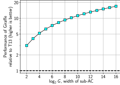
FIGURE 17— Effect of Giraffe’s protocol optimizations (§3.1). We compare the performance of Giraffe’s prover to T13’s prover by counting field multiplications for a generic AC (§6.1) with number of sub-AC copies N = 2^{10} , fraction of multipliers \delta = 0.5 , and depth d = 20 . Giraffe’s protocol improves over T13 by about a factor of \log G . This improvement is essentially insensitive to N , \delta , and d . Comparing field additions gives a similar result.
